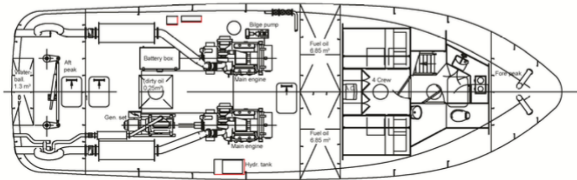
Below Maindeck
