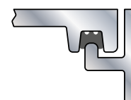
S-K Steel deck ring with knife edge seal
