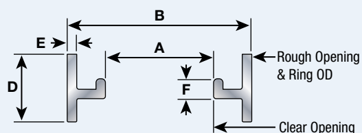
S-C Steel Deck Ring with Compression Seal
